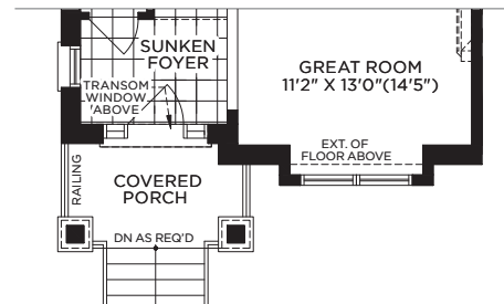
End Mod Elev B Main Floor
