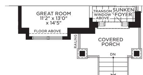
End Elev B Main Floor
