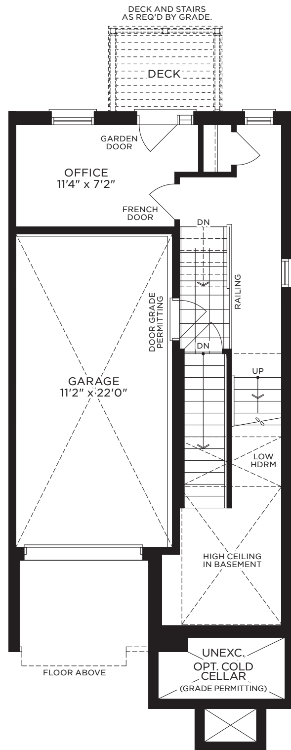
End Elev B Lower Floor
